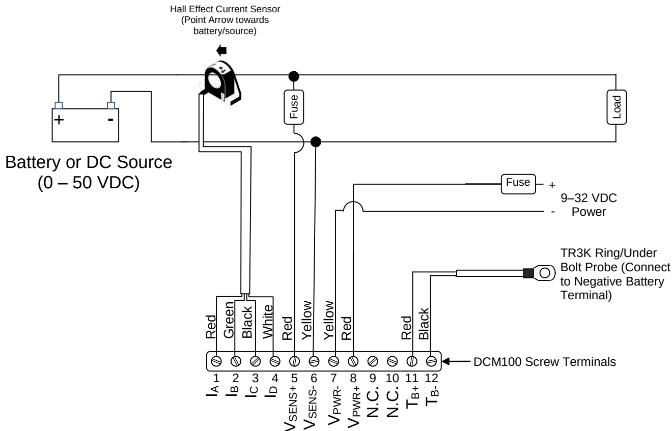
Figure 3 – Connection Diagram
